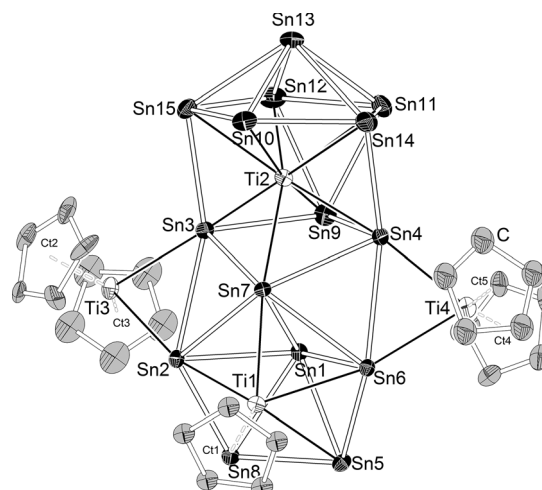
Figure 4. Structure of [\text{Ti}_4\text{Sn}_{15}\text{Cp}_5]^{7-} ( 7a ) in [\text{K}([\text{18}]\text{crown-6})]_6(\eta^5\text{-Cp})_4[\text{K}([\text{18}]\text{crown-6})(\text{NH}_3)_2]_2[\text{Cp}_5\text{Ti}_4\text{Sn}_{15}]_2(\text{NH}_3)_{40} ( 7 ). Atoms are drawn at the 50% probability level at 120 K. Hydrogen atoms are omitted for clarity. Ct represents the center of the coordinating Cp ligands.
